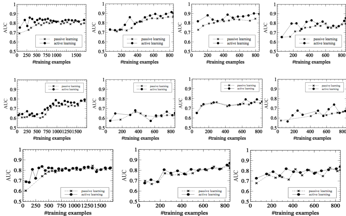
Figure 2. Results of output quality using passive and active learning, measured using AUC, vs. number of training labels. Each column corresponds to one phase starting from S1 (from left) to S4 (In the Oklahoma dataset there are only 3 phases). Datasets are: Joplin (top), Sandy (middle) and Oklahoma (bottom).
